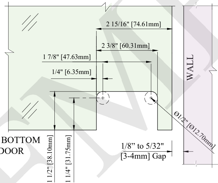
GLASS FABRICATION TEMPLATE
